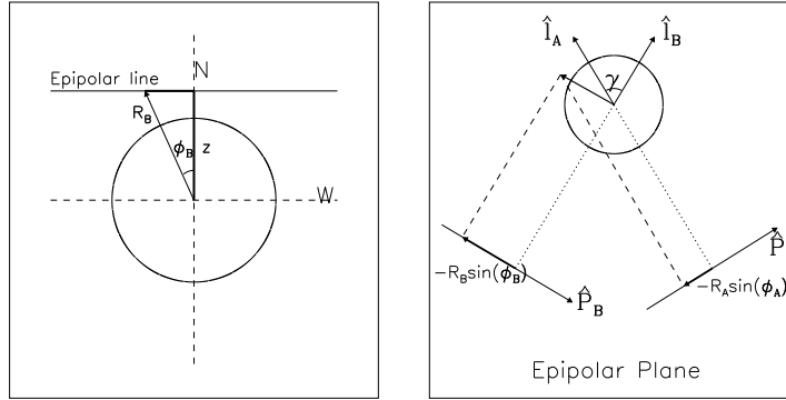
Figure 2. Left panel: Sketch of the projected position of the moving feature on COR1 B image. The feature is at a distance R_B from the Sun center and its ecliptic position angle is \phi_B . The epipolar line is represented by the solid horizontal line. Right panel: Sketch of the epipolar plane containing the moving feature. The moving feature is represented by the vector ending at the intersection of the two dashed lines. The two COR1 A and B images are represented by \hat{\mathbf{P}}_A and \hat{\mathbf{P}}_B vectors. \hat{\mathbf{I}}_A and \hat{\mathbf{I}}_B are perpendicular on \hat{\mathbf{P}}_A and \hat{\mathbf{P}}_B respectively. \gamma is the separation angle between the two spacecraft. The circles in the two panels represent the solar disk.
