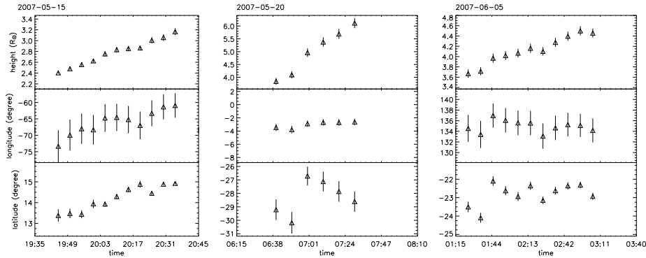
Figure 4. Plots of height (upper panels), ecliptic longitude (middle panels) and ecliptic latitude (lower panels) with time for the identifiable features (indicated by arrows) of the three events shown in Figure 1. The errors are calculated from the initially estimated errors of R and \phi .
