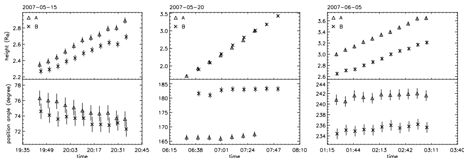
Figure 3. Plots of height (upper panels) and ecliptic position angle (lower panels) versus time for the objects indicated by arrows in Figure 1. The ecliptic position angle of the tracked object is measured from the north ecliptic pole, counterclockwise. The errors estimate the uncertainties in selecting the tracked objects: 1^\circ ( i.e. , three pixels at 1.4 R_\odot and nine pixels at 4 R_\odot ) in azimuthal direction and 0.038 R_\odot (5 pixels) in radial direction.
