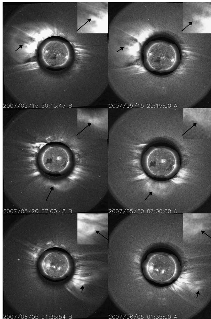
Figure 1. SECCHI-EUVI and SECCHI-COR1 combined images taken on 15 May (upper panels), 20 May (middle panels) and 5 June (lower panels), from both A (right) and B (left) spacecraft. The COR1 images show the white light total brightness corona from 1.4 to 4 R_{\odot} and EUVI images show the UV corona at 19.5 nm. Arrows indicate the traced features. A zoomed region containing the traced feature is shown in the upper right corner of each image.
